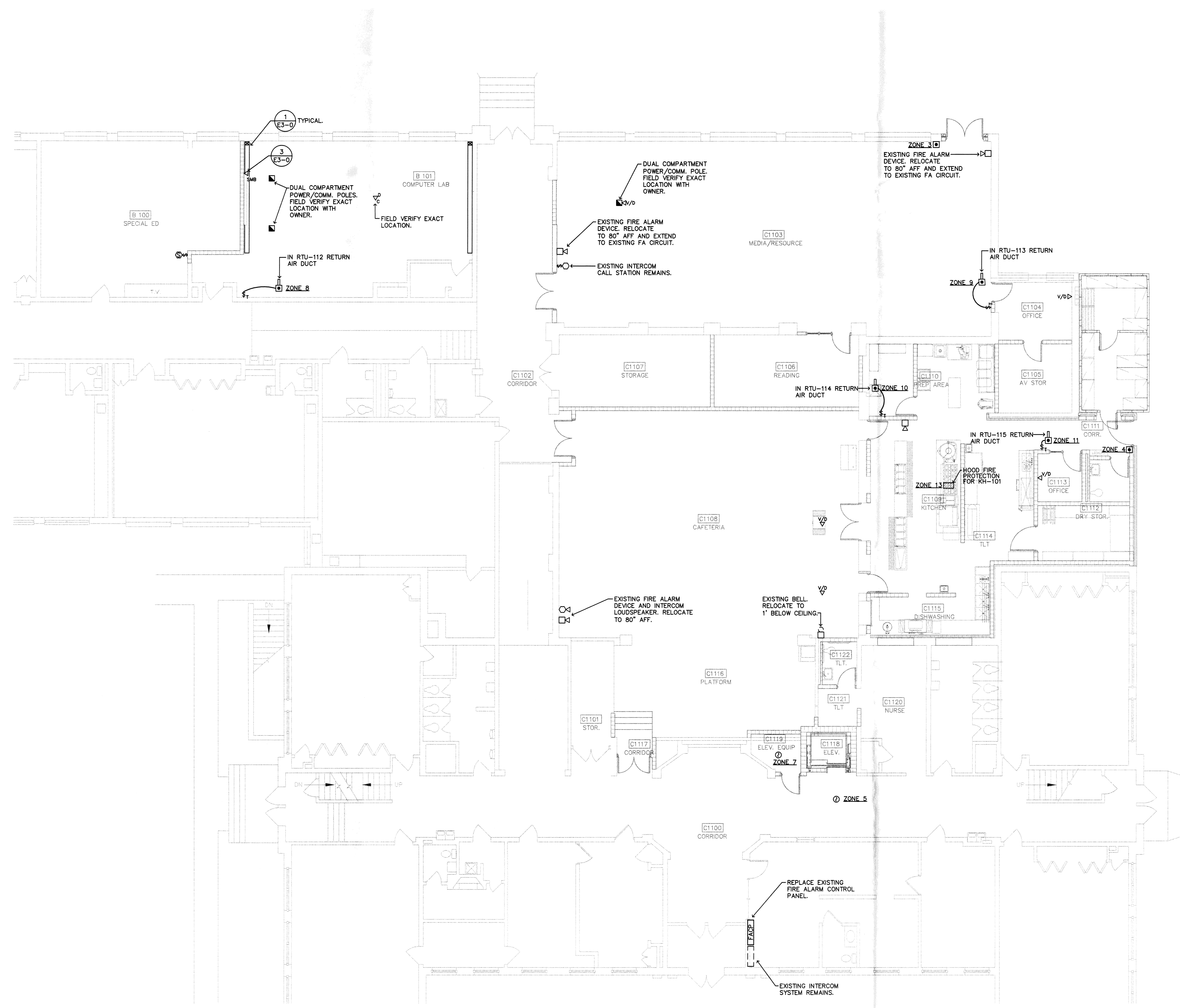
FIRE ALARM AND COMMUNICATIONS PLAN - AREA 'B' & 'C' SCALE: 1/8" = 1'-0" PROJECT NORTH
