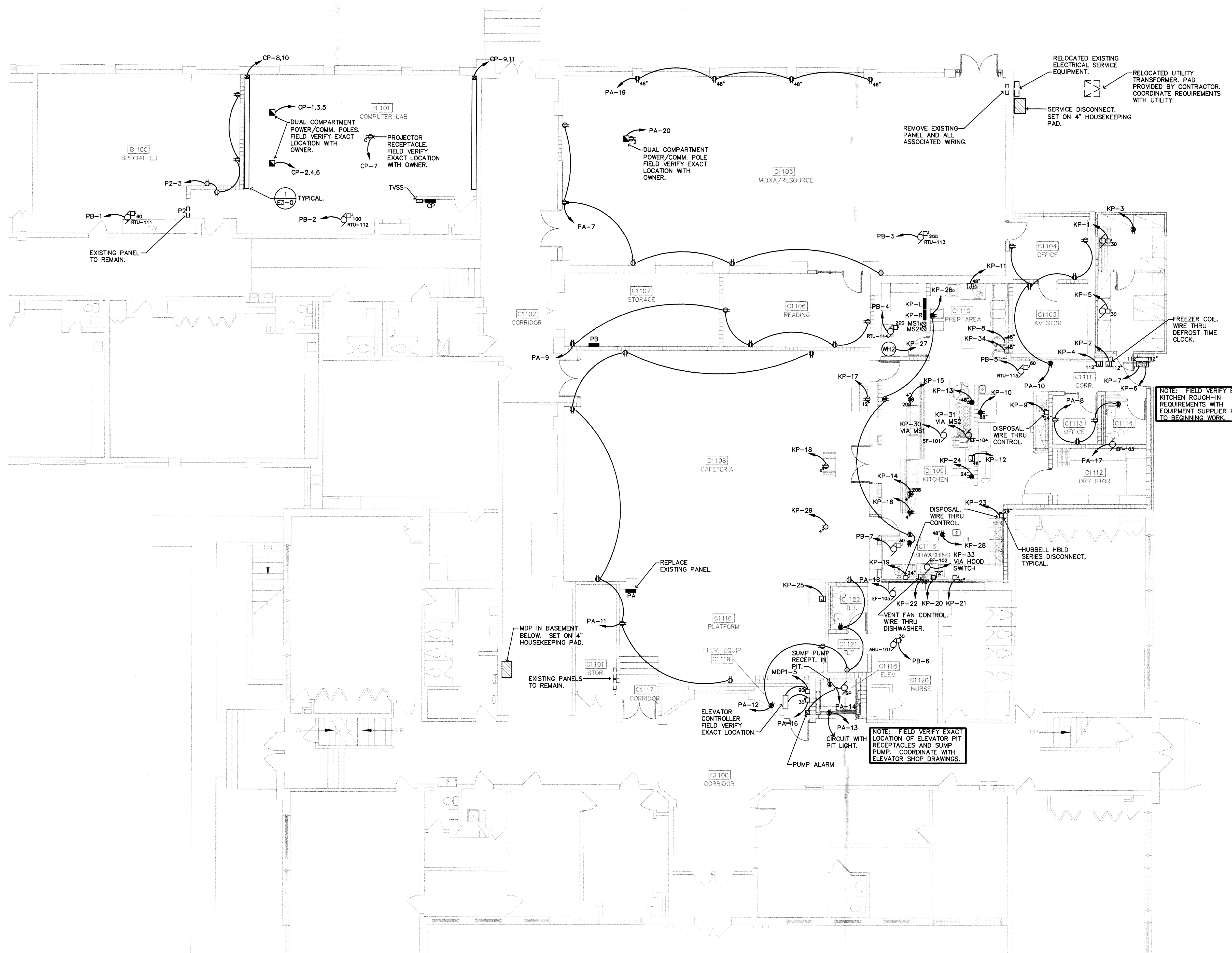
POWER PLAN - AREA 'B' & 'C' SCALE: 1/8" = 1'-0" PROJECT NORTH
