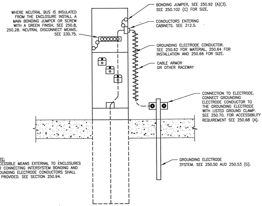
GROUNDING DIAGRAM NOT TO SCALE
