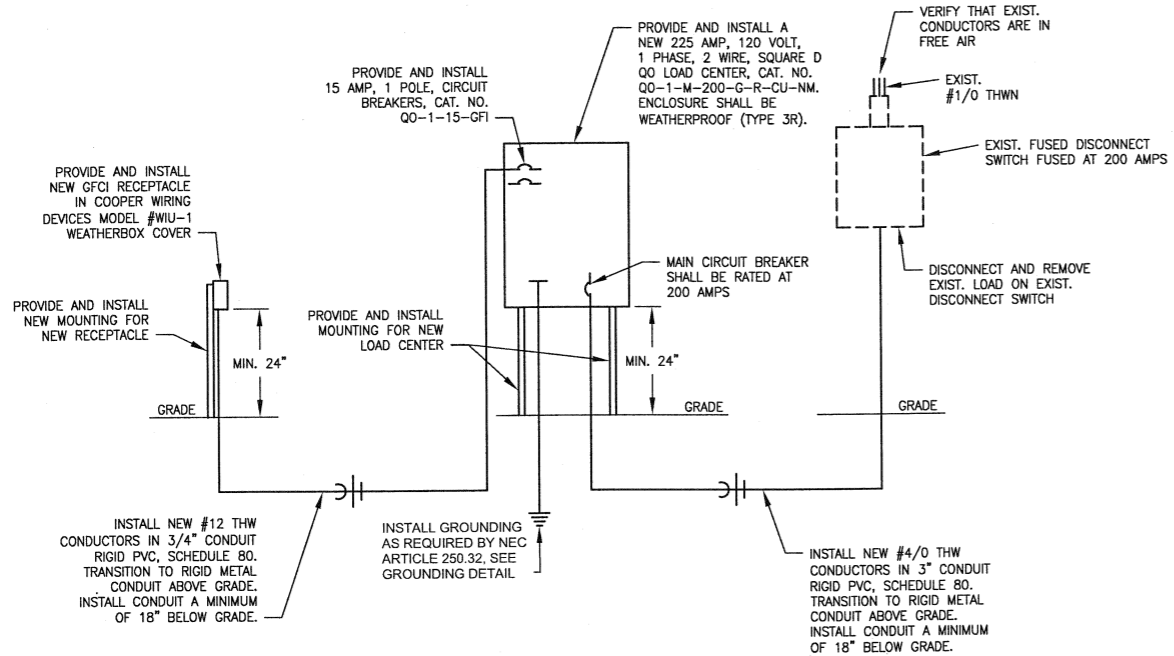
ELECTRICAL DIAGRAM NOT TO SCALE
