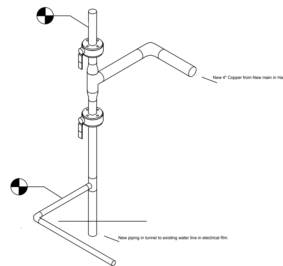
Detail 1.1
